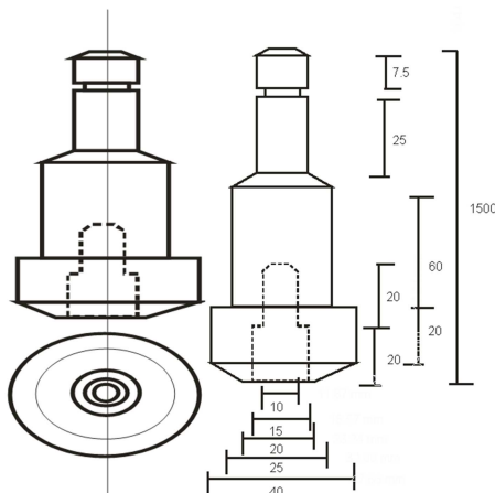
Appendix 1. Mechanical Engineering Component (Stud), Instruction: All Dimension in Millimeters.
