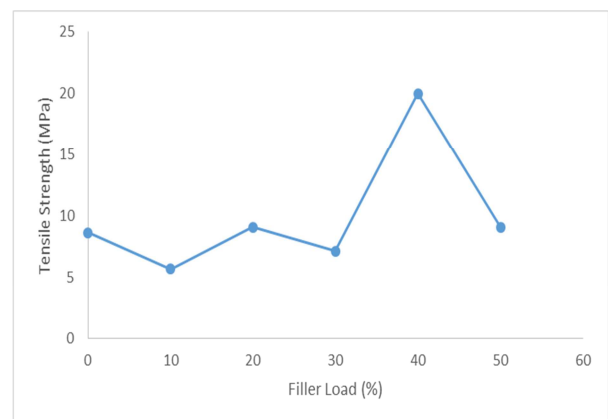
Fig. 6. Effect of filler loading on the tensile strength of polypropylene composites.
