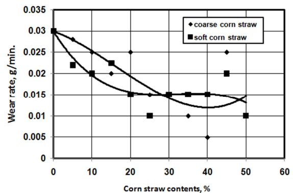
Fig. 4. Effect of corn straw content on the rate of wear of polyester composites.
