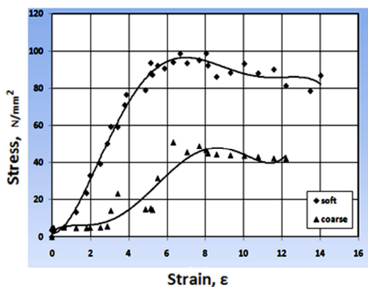
Fig. 12. Stress – strain curve for polyester composite filled with 30 wt. % jasmine leaves.
