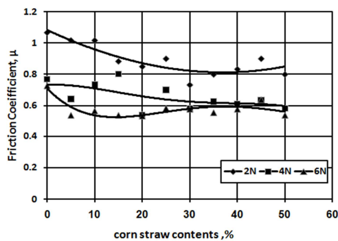
Fig. 2. Effect of coarse corn straw particles on the friction coefficient of polyester composites.
