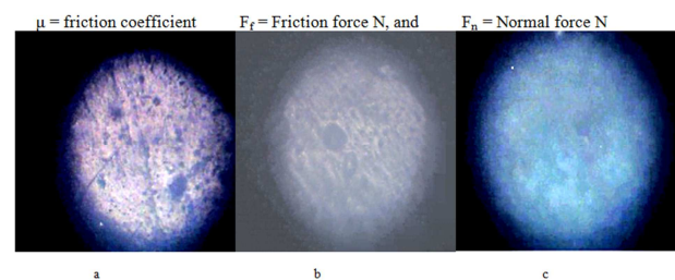
Fig. 1. a) unfilled polyester, b) polyester reinforced by soft particles and c) polyester reinforced by coarse particles.
