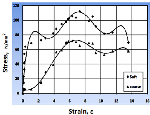
Fig. 11. Stress – strain curve for polyester composite filled with 5 wt. % jasmine leaves.
