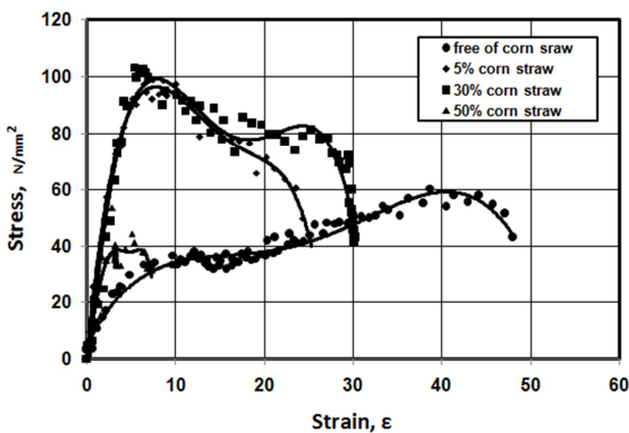
Fig. 5. Effect of coarse corn straw particles on the stress-strain curve of polyester composites.
