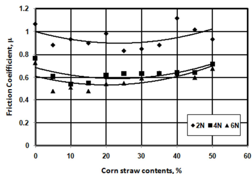
Fig. 3. Effect of soft corn straw particles on the friction coefficient of polyester composites.
