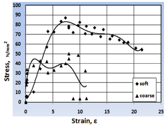
Fig. 13. Stress – strain curve for polyester composite filled with 50 wt. % jasmine leaves.
