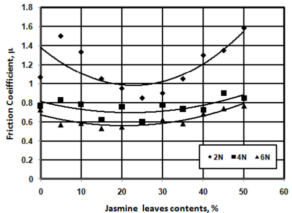
Fig. 8. Effect of coarse jasmine leaves particles on the friction coefficient of polyester composites.
