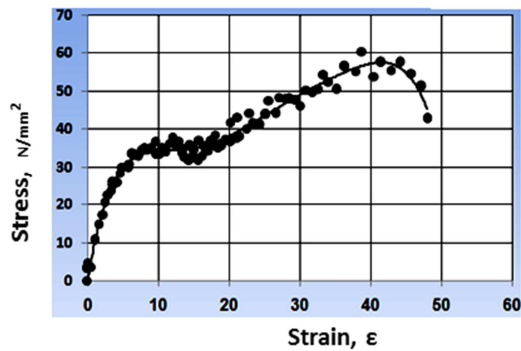
Fig. 10. Stress – strain curve for polyester free of jasmine leaves.
