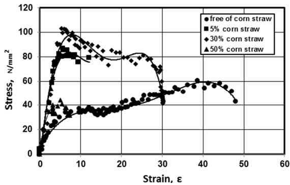
Fig. 6. Effect of soft corn straw particles on the stress-strain curve of polyester composites.
