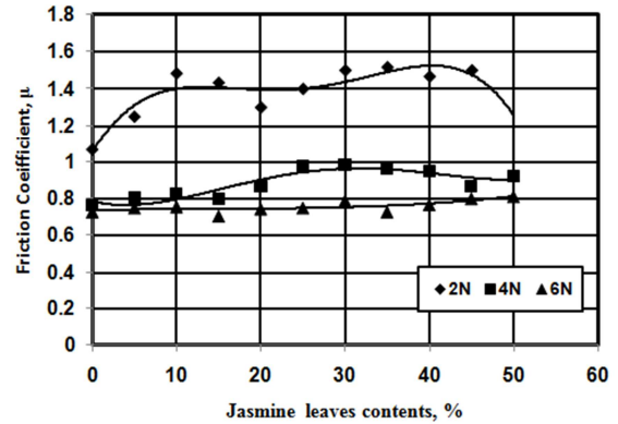
Fig. 7. Effect of soft jasmine leaves particles on the friction coefficient of polyester composites.
