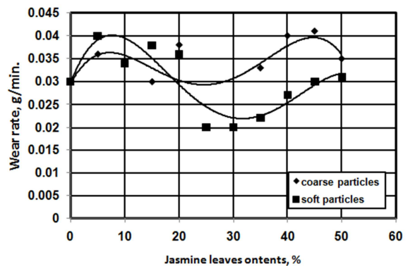
Fig. 9. Effect of jasmine leaves particles on the wear rate of polyester composites.
